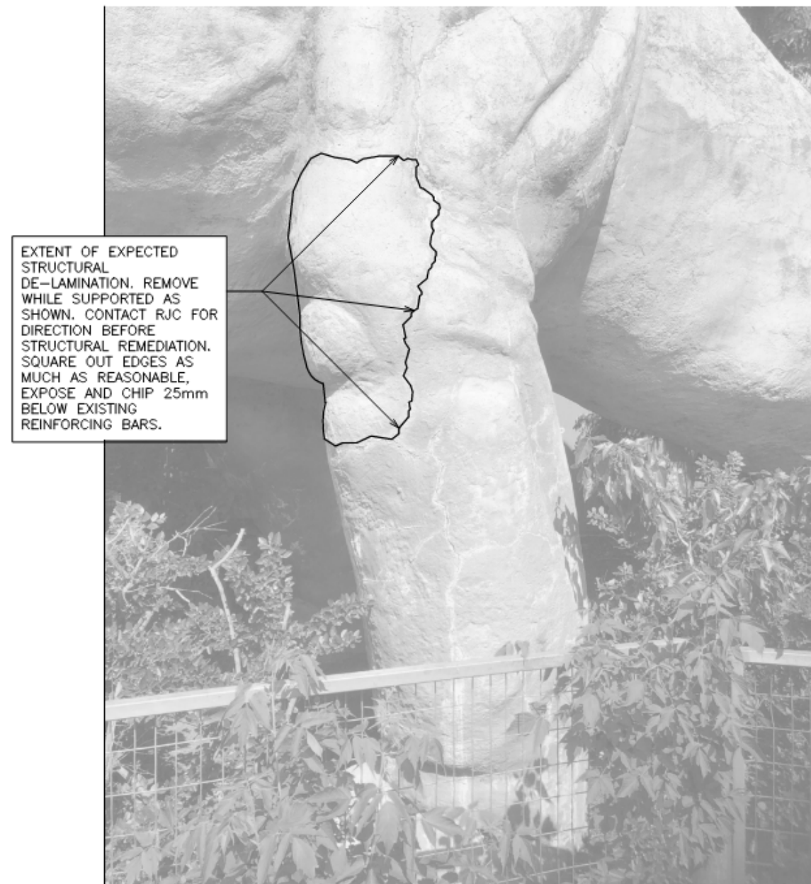
3 KNEE REPAIR EXTENTS S400 NTS
