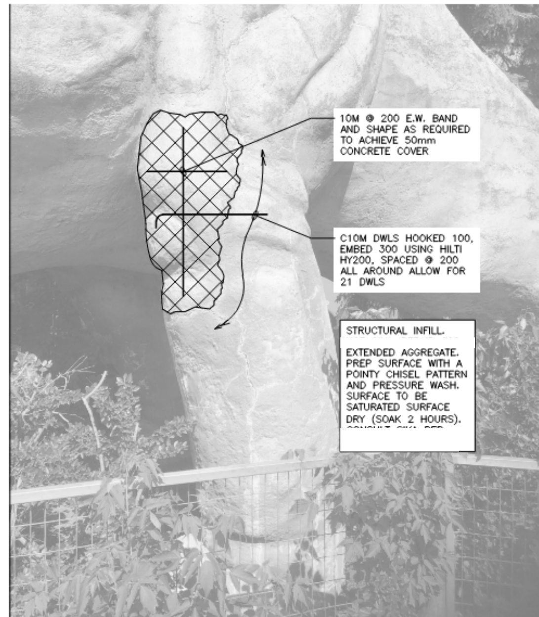
4 KNEE REPAIR DETAIL S400 NTS
