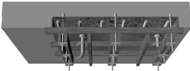
Formwork complete ready for pumpline hookup
