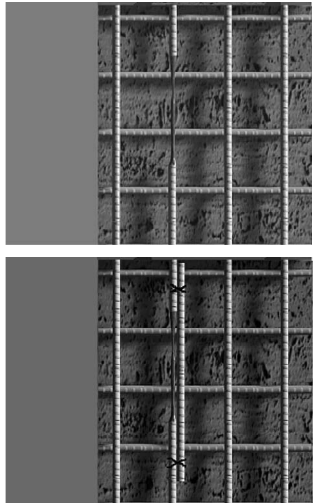
Fig. 1—Lapping of supplemental reinforcing.
