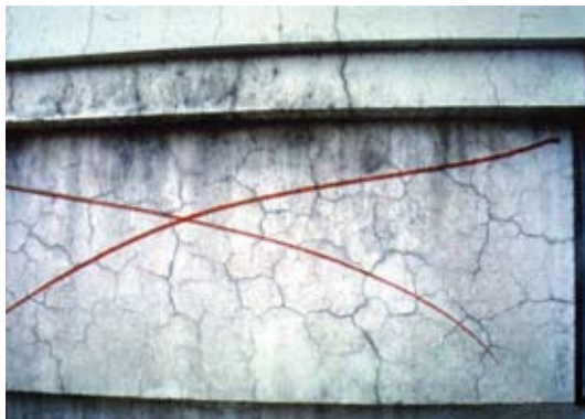
Fig. 3: Heavy crazing in a cast stone façade panel
